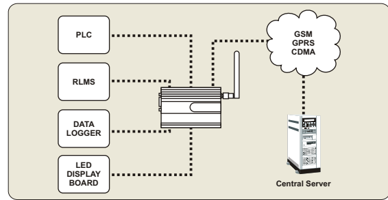
Application Diagram
